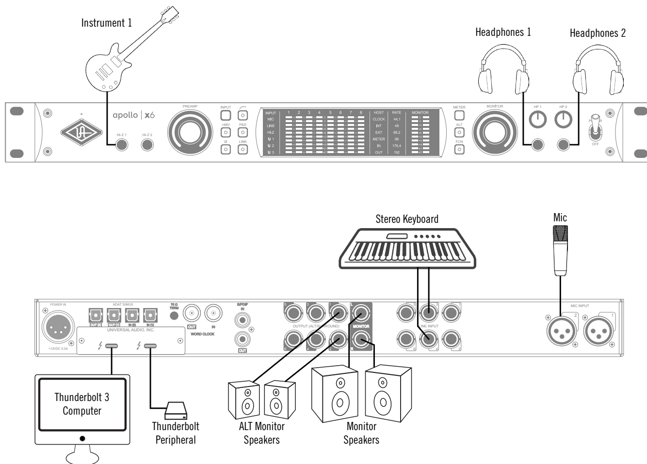
Typical Apollo x6 connections
