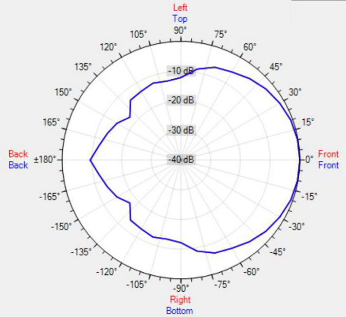
Data Shown: MP16 (Apart Audio) Display Parameters: Frequency: 2000Hz (1/24th Octave)
