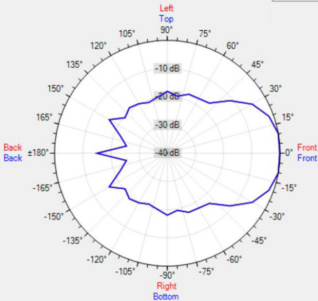
Data Shown: MP16 (Apart Audio) Display Parameters: Frequency: 4000Hz (1/24th Octave)
