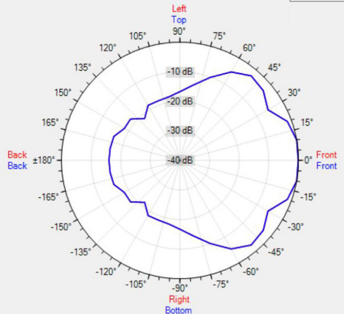
Data Shown: MP16 (Apart Audio) Display Parameters: Frequency: 8000Hz (1/24th Octave)
