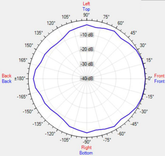
Data Shown: MP16 (Apart Audio) Display Parameters: Frequency: 1000Hz (1/24th Octave)
