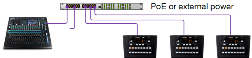
From rear panel dSNAKE port
