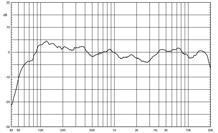
WD12A - preset FOH
