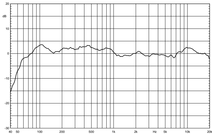
WD15A - preset MONITOR
