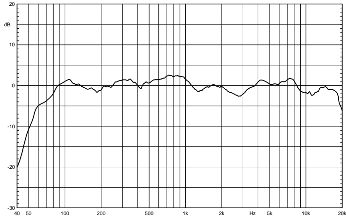
WD12A - preset MONITOR
