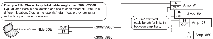
Figure 7.7.5b: NomadLink closed loop configuration
