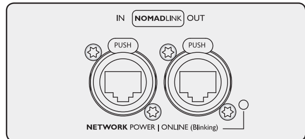
Figure 7.7.1: NomadLink Network RJ45 connectors
