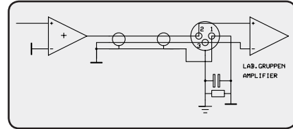
Figure 7.4.2: Unbalanced XLR wiring schematic
