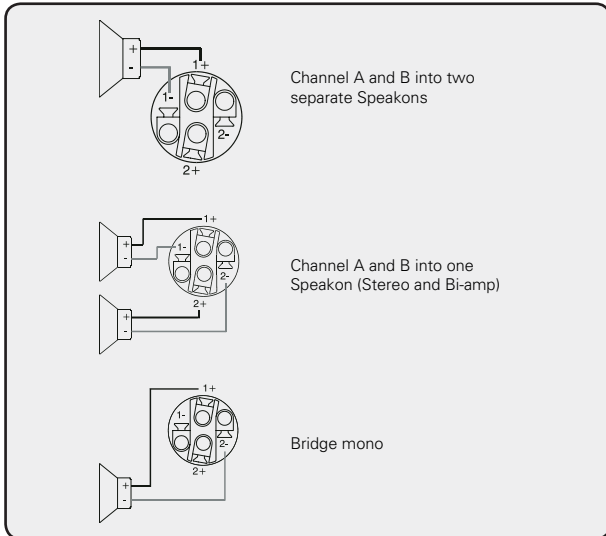
Figure 7.4.3c: Speakon wiring schematic
