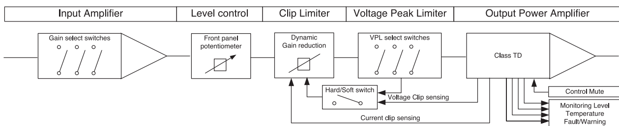
Figure 7.3.1: FP+ Series signal flow diagram
