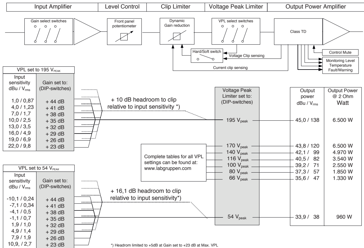
Figure 7.3.2: FP 13000 VPL and GAIN settings
