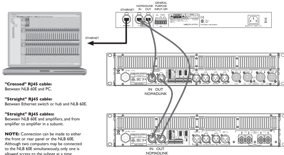
Figure 6.3: NomadLink network wiring configuration
