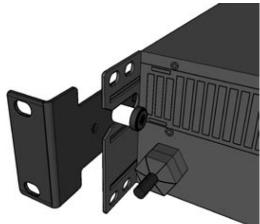
Figure 5.2c: Use tube for slide-on installation.
