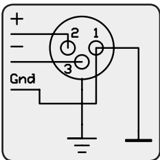
Figure 7.4.1c: Balanced XLR wiring schematic
