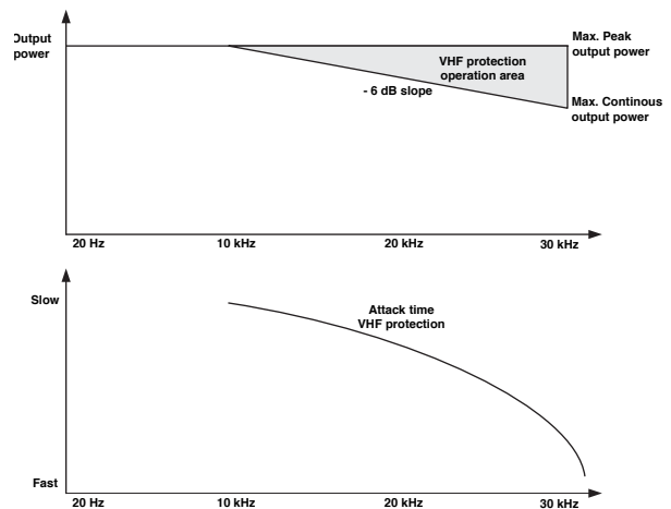
Figure 7.5.3: VHF protection attack time vs output power/frequency
