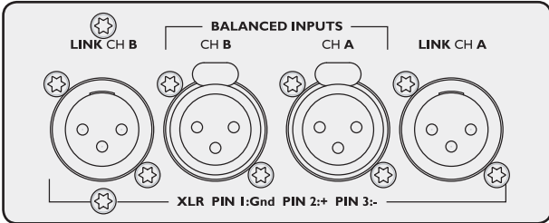
Figure 7.4.1a: Audio inputs and loop-thru connectors - two-channel models
