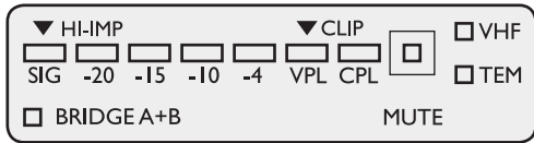
Figure 7.6.1: Front panel LED field (per-channel)
