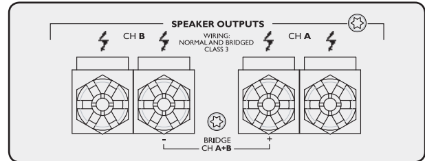
Figure 7.4.4a: Binding Post outputs - two-channel models
