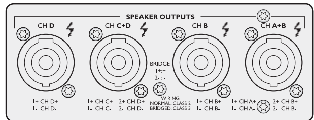
Figure 7.4.3b: Speakon outputs - four-channel models
