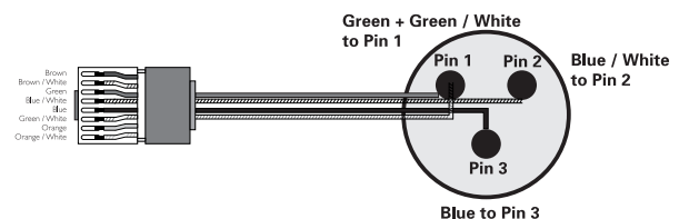
Figure 7.7.2: NomadLink RJ45 to XLR wiring schematic
