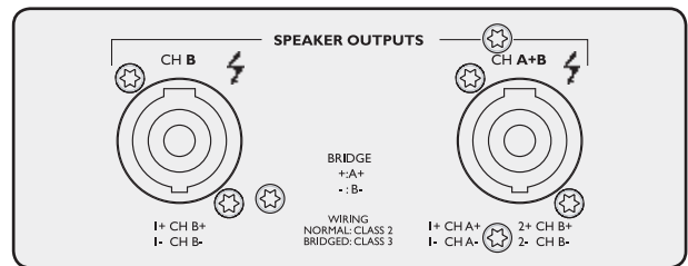
Figure 7.4.3a: Speakon outputs - two-channel models
