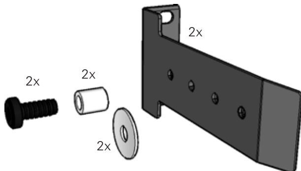
Figure 5.2a: Rear support mounting hardware
