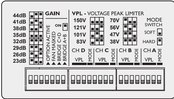
Figure 6.2.2a: Rear panel DIP-switch field
