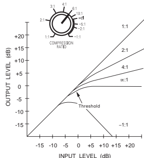
Figure 3: Ratio Control and Infinity+ (Negative) Ratios
